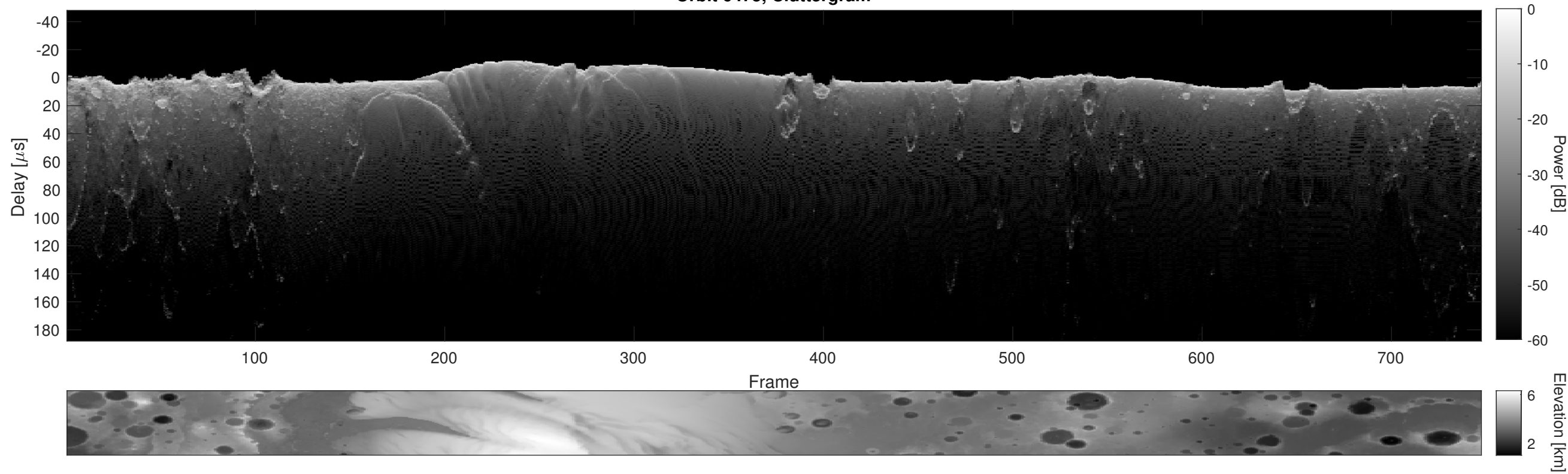
Orbit 6475, Cluttergram
