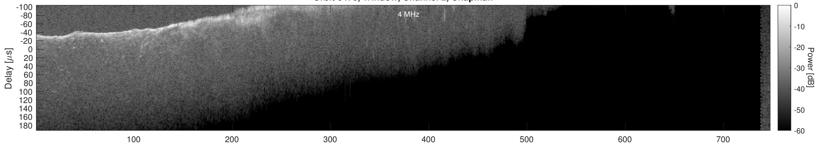
Orbit 6476, Window, Channel 2, Optimized
