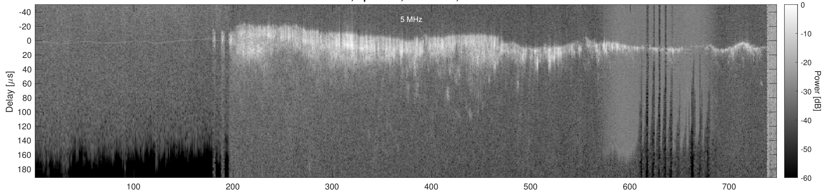
Orbit 6476, Optimized, No Window, Channel 2
