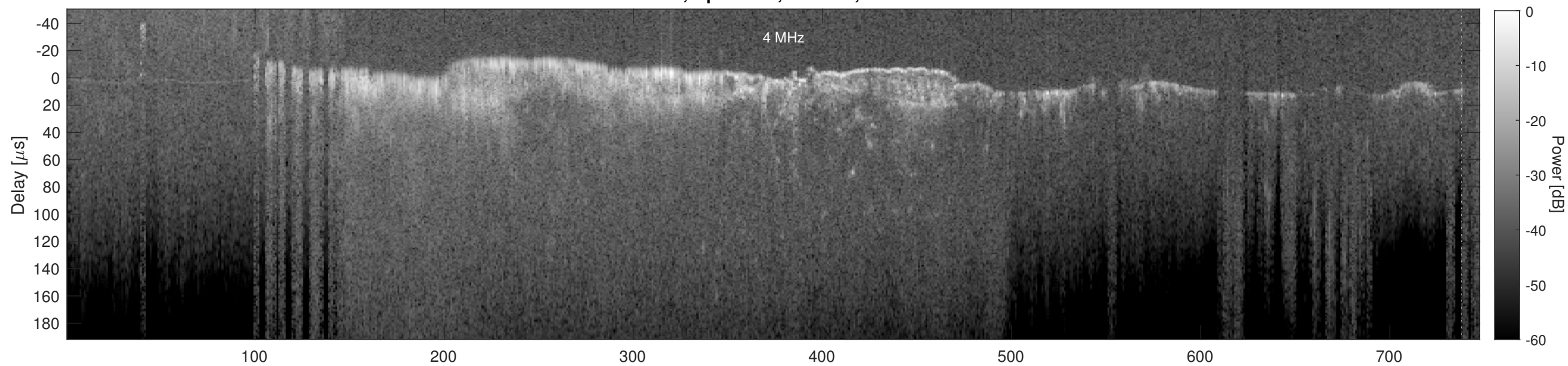
Orbit 6476, Cluttergram
