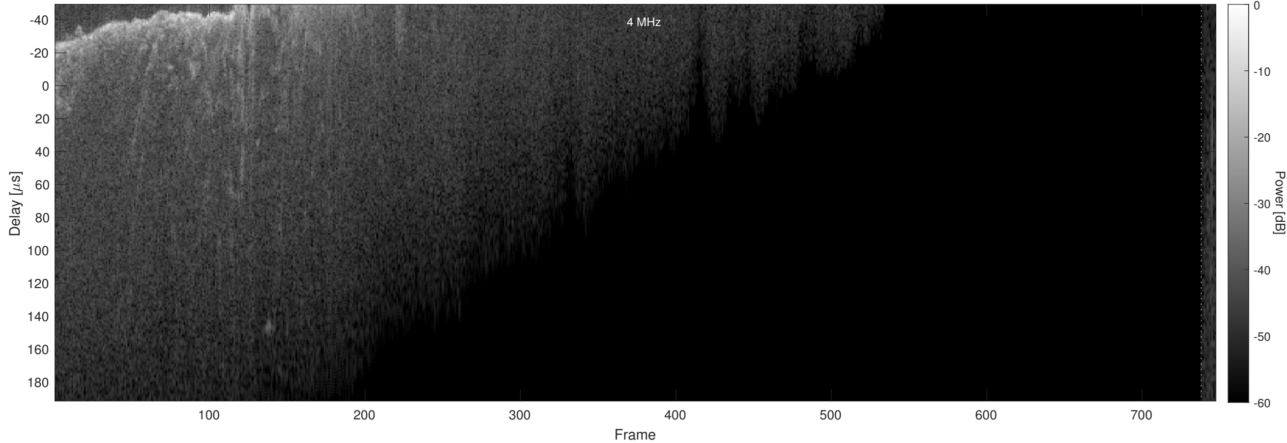
Orbit 6479, Chapman, No Window, Channel 2
