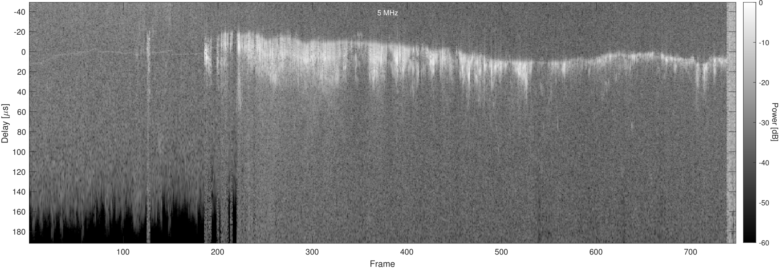
Orbit 6479, Optimized, No Window, Channel 2
