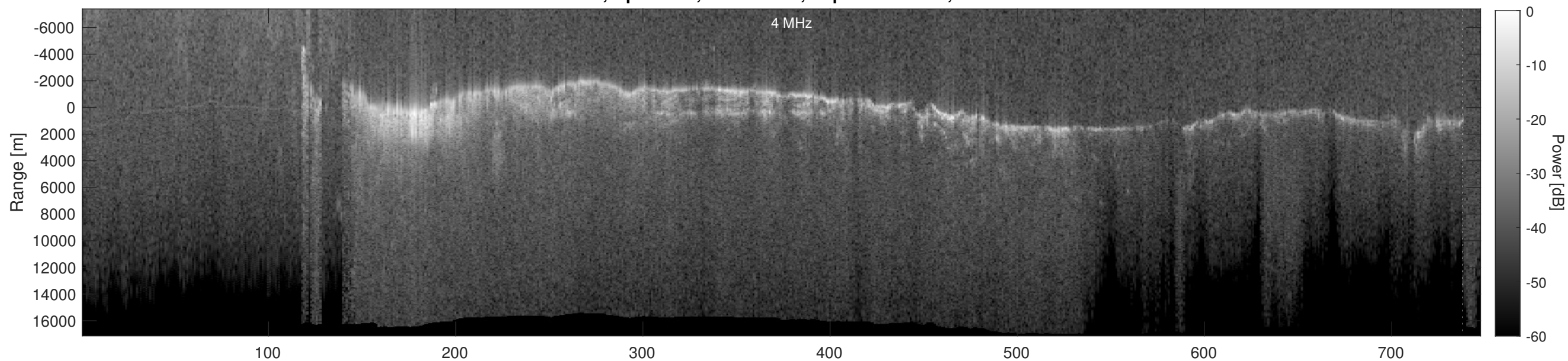
Orbit 6479, Depth-Corrected Cluttergram
