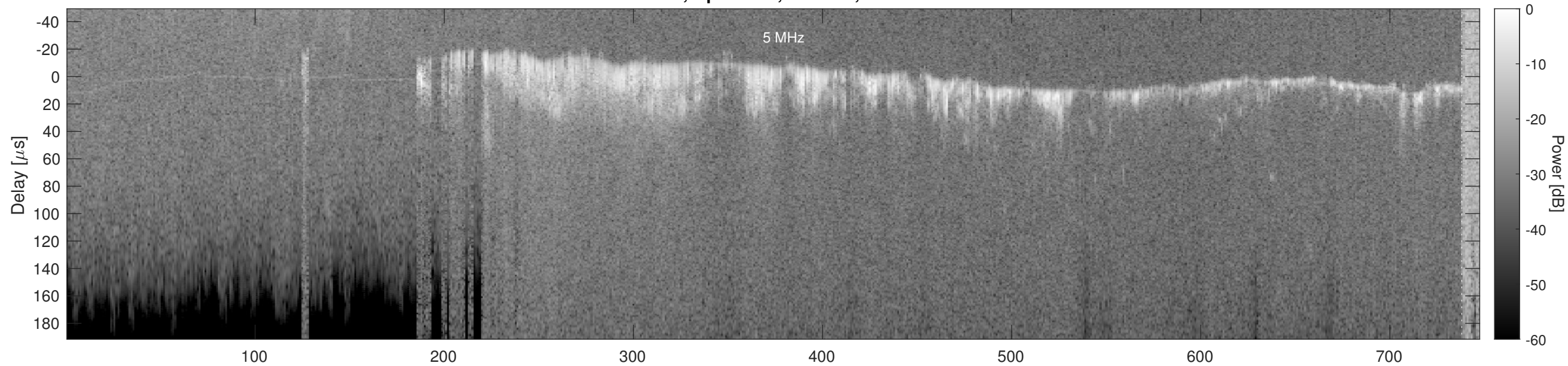
Orbit 6479, Optimized, Window, Channel 2
