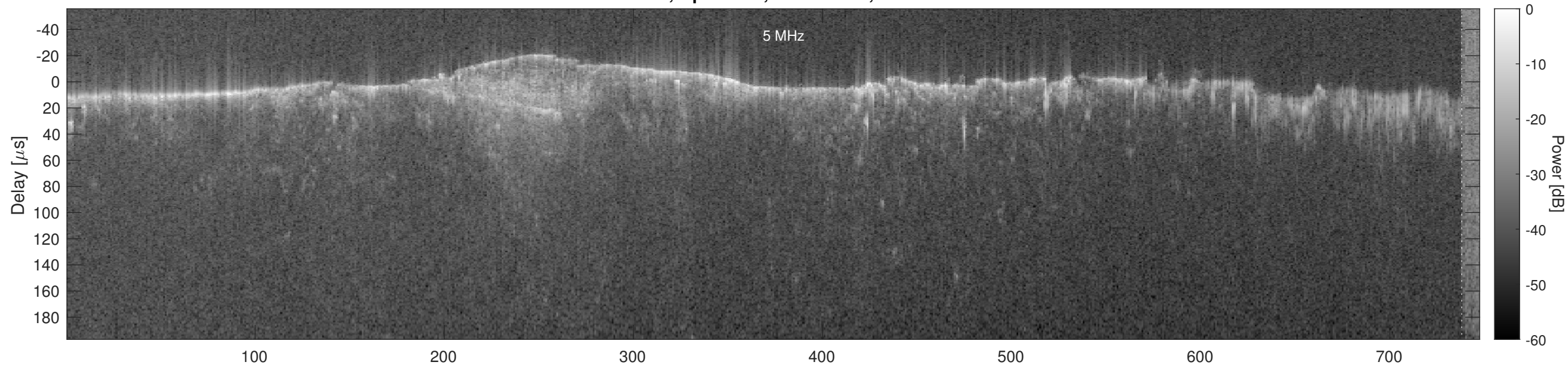
Orbit 6480, Optimized, No Window, Channel 2
