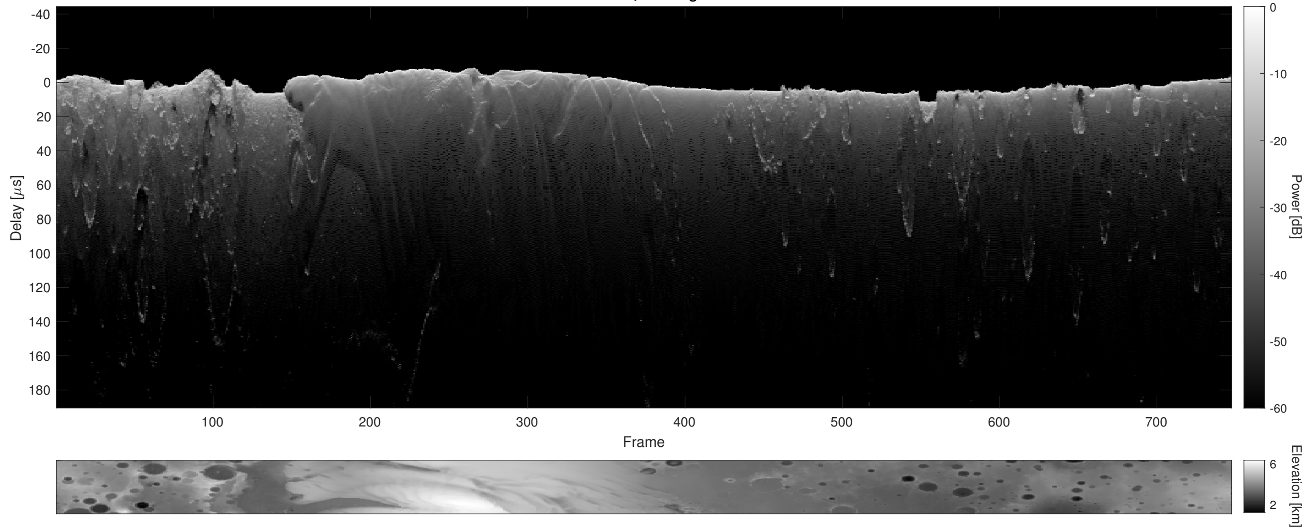
Orbit 6482, Cluttergram
