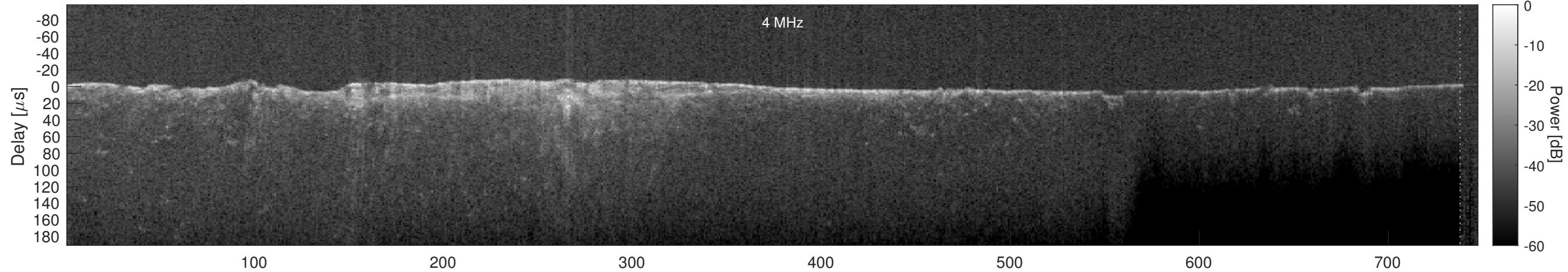
Orbit 6482, Cluttergram
