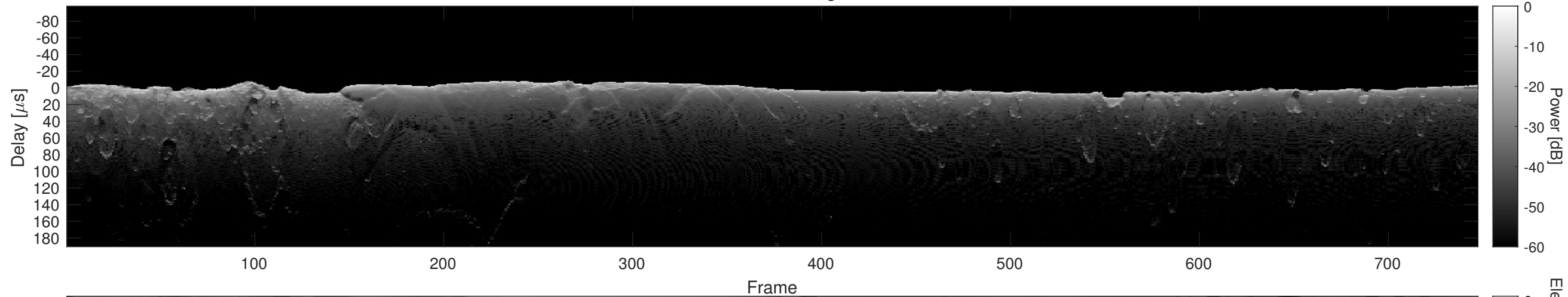
Orbit 6482, Cluttergram
