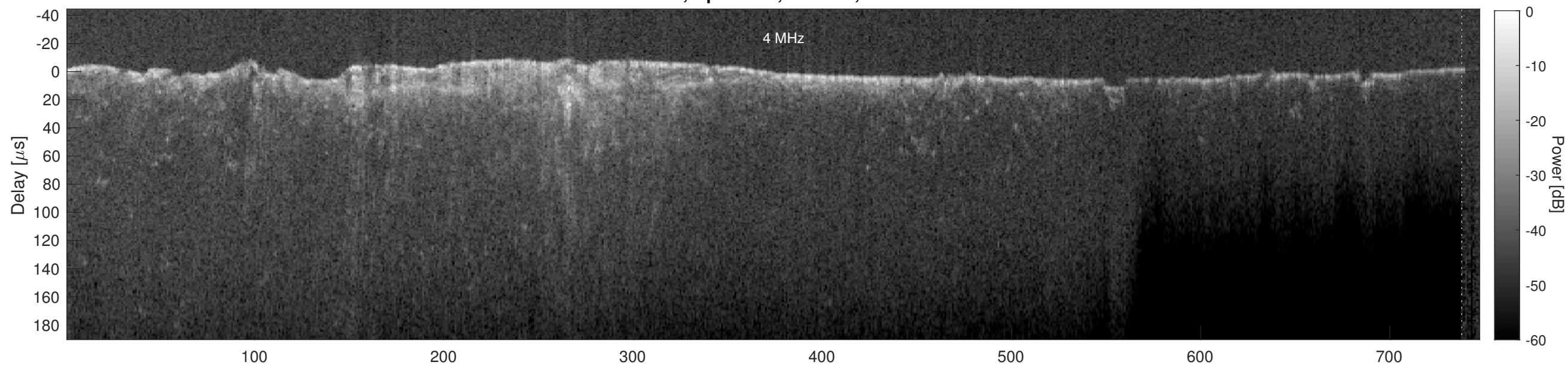
Orbit 6482, Cluttergram
