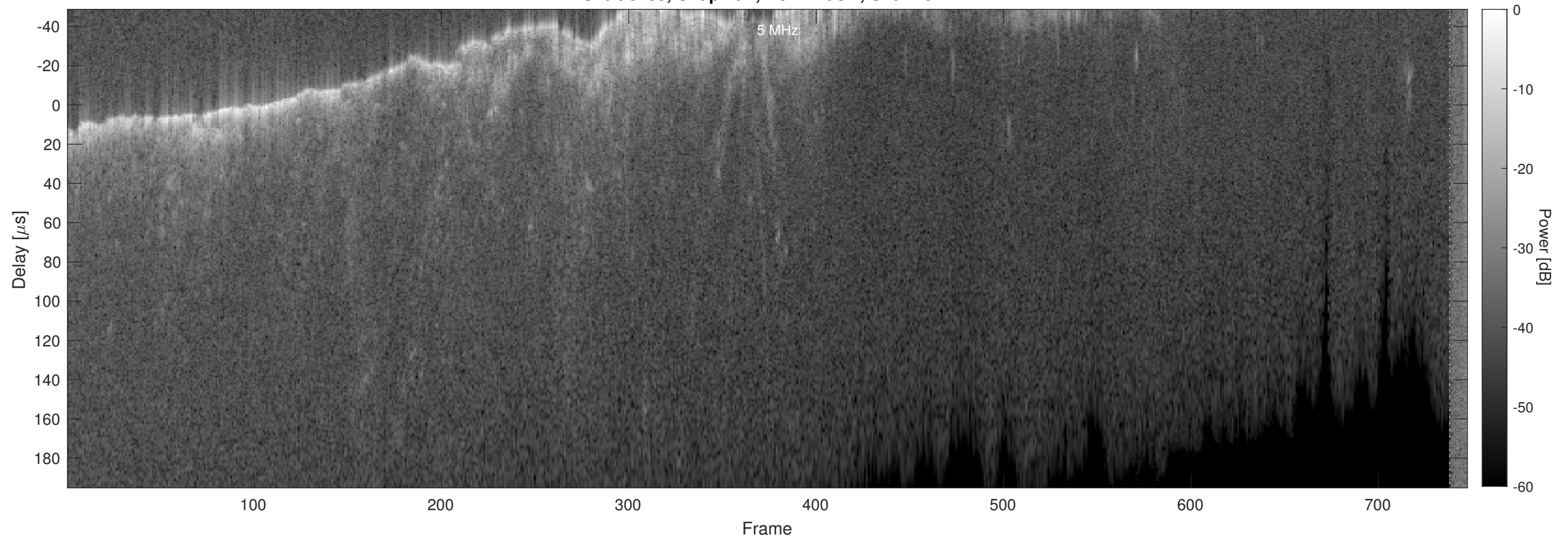
Orbit 6483, Chapman, No Window, Channel 2
