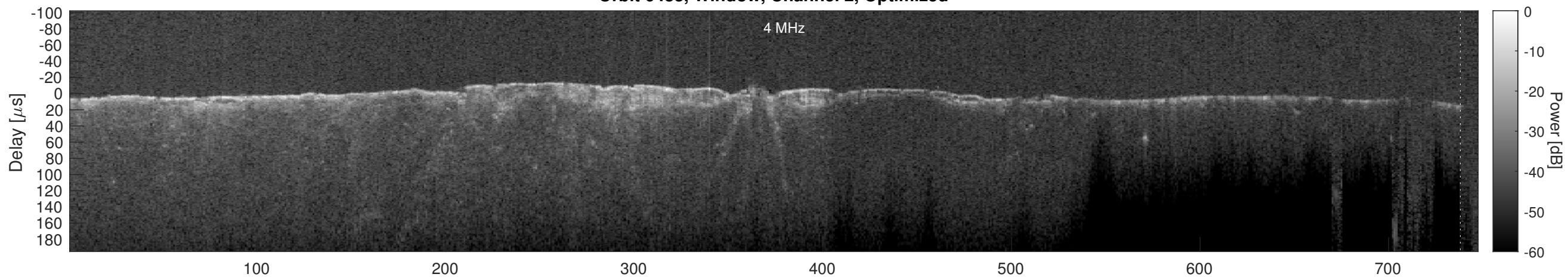
Orbit 6483, Cluttergram
