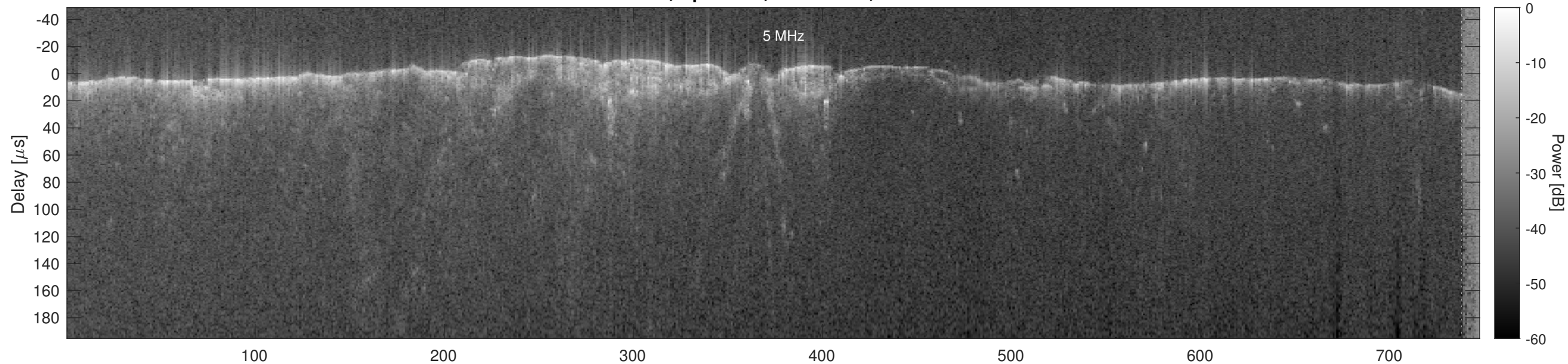
Orbit 6483, Optimized, No Window, Channel 2
