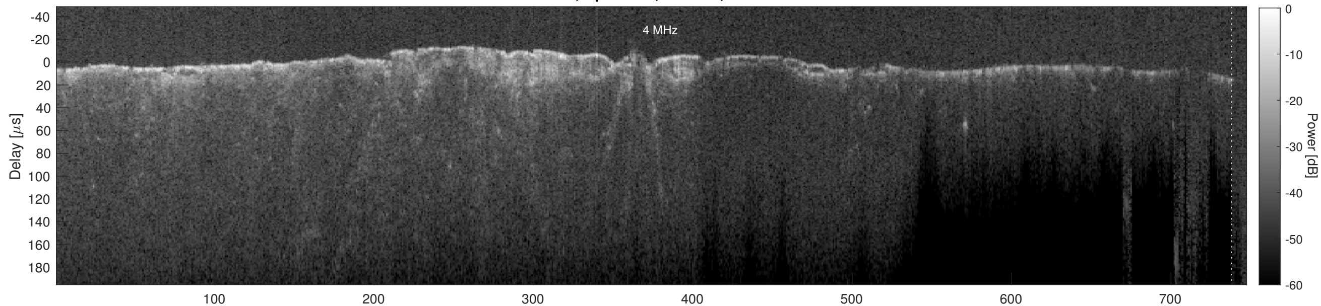
Orbit 6483, Cluttergram
