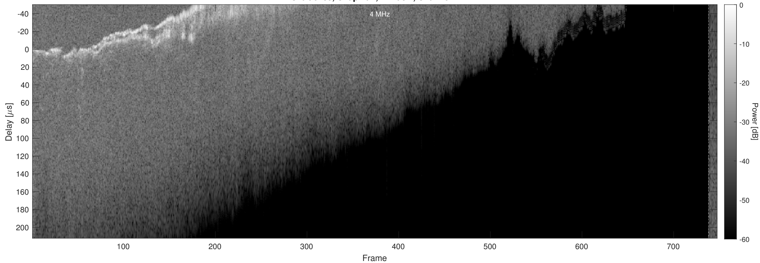
Orbit 6485, Chapman, Window, Channel 2
