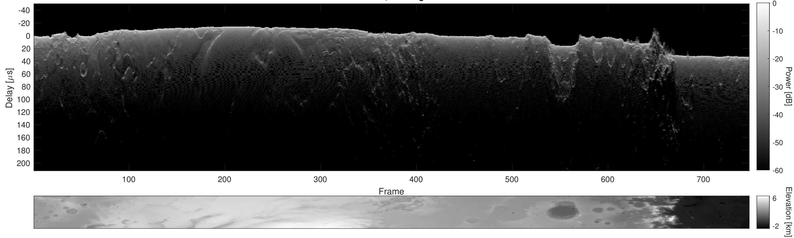
Orbit 6485, Cluttergram
