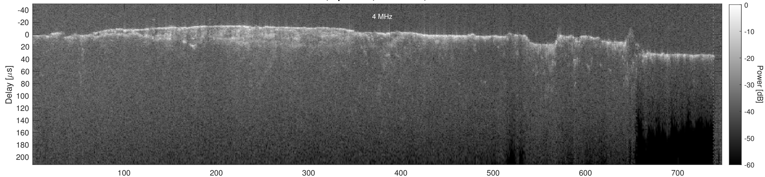
Orbit 6485, Cluttergram
