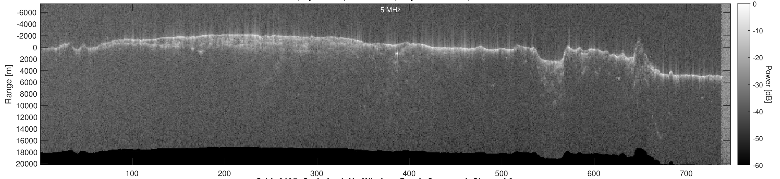
Orbit 6485, Optimized, No Window, Depth-Corrected, Channel 2
