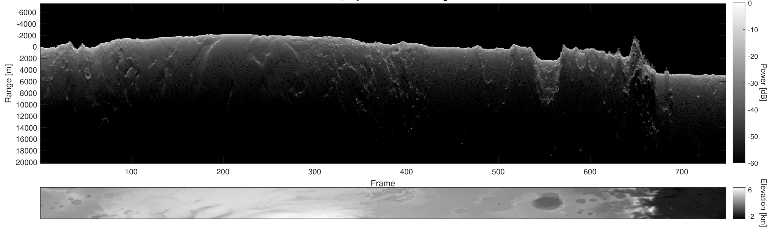
Orbit 6485, Depth-Corrected Cluttergram
