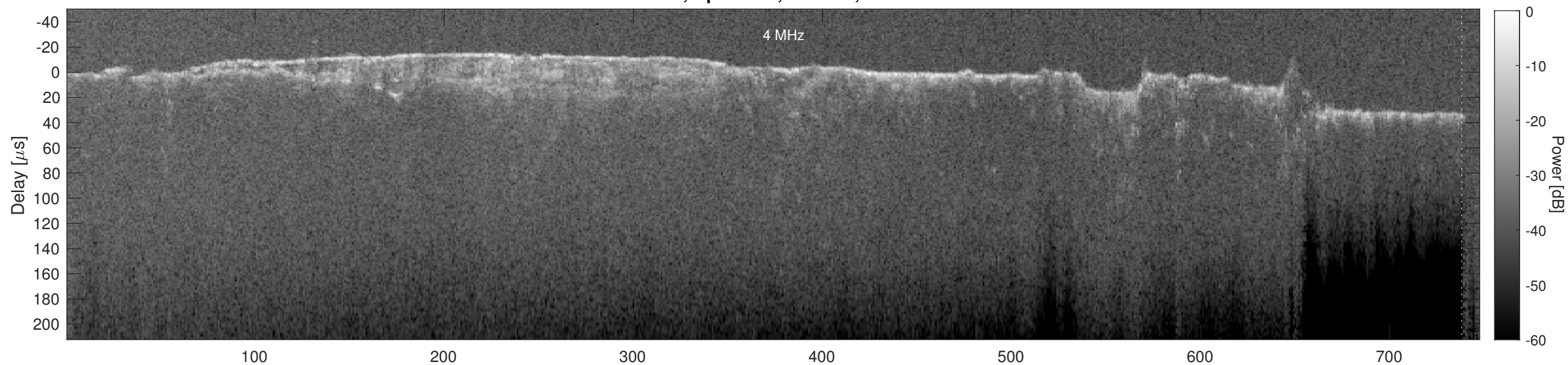
Orbit 6485, Cluttergram
