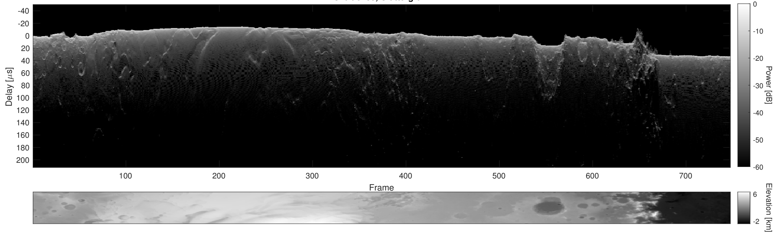
Orbit 6485, Cluttergram
