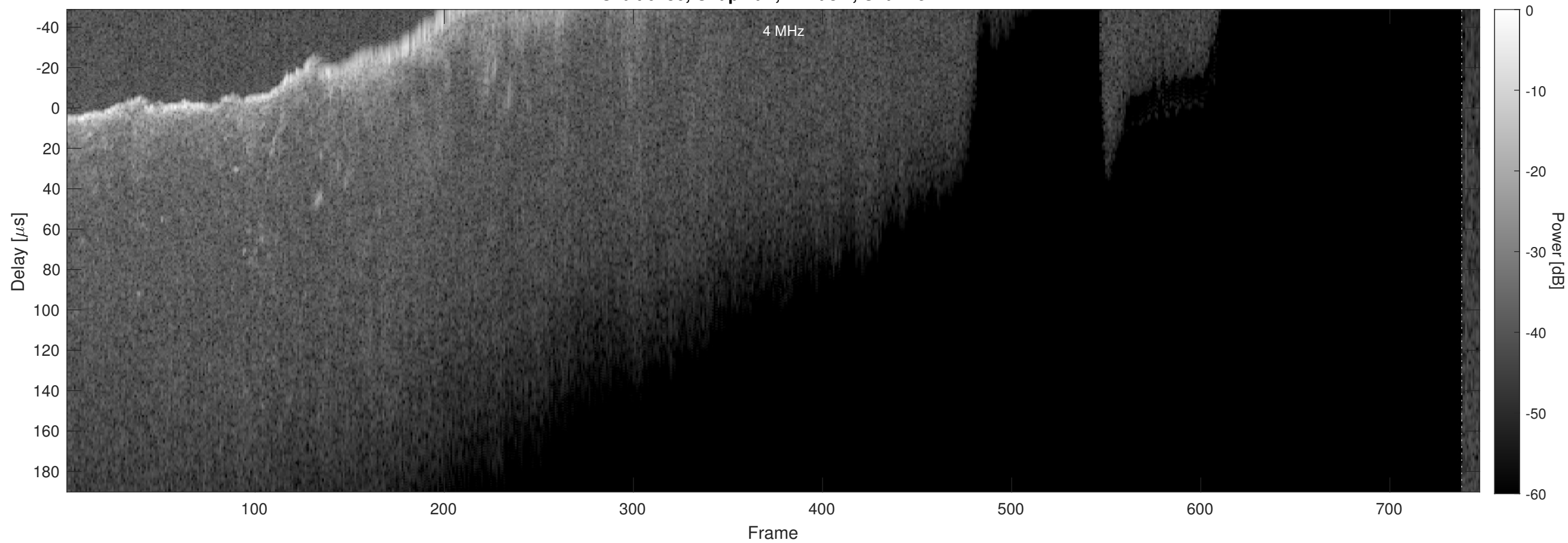
Orbit 6486, Chapman, Window, Channel 2
