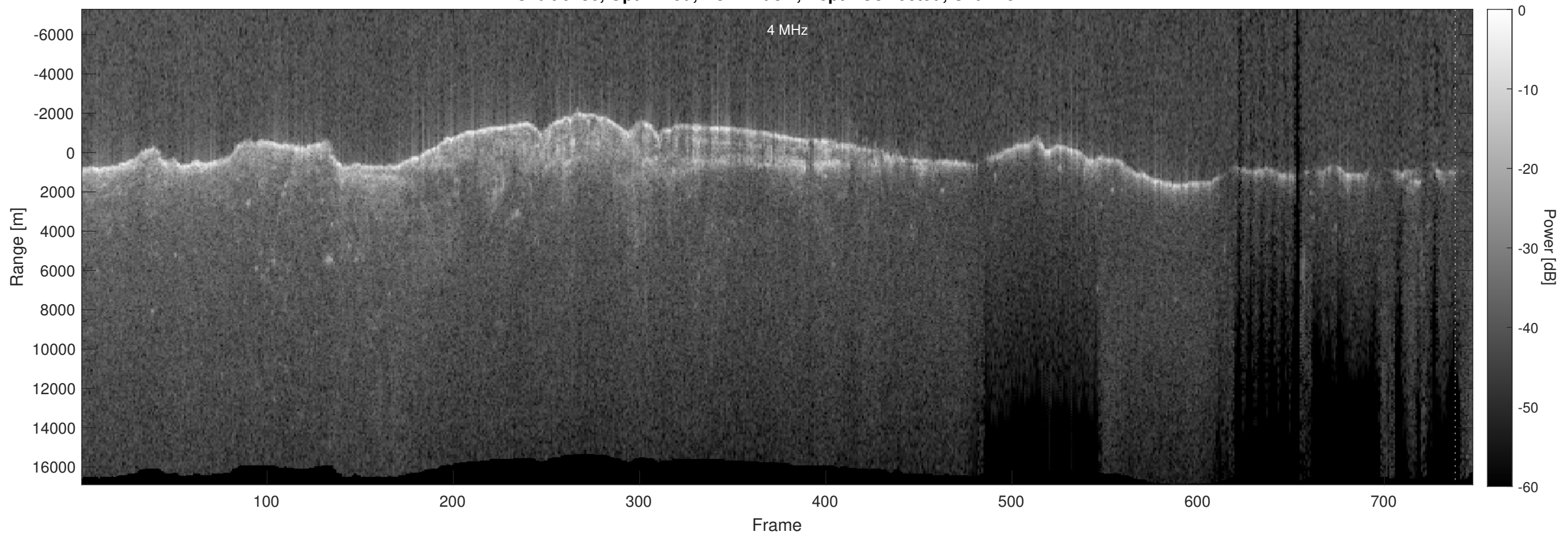
Orbit 6486, Optimized, No Window, Depth-Corrected, Channel 2
