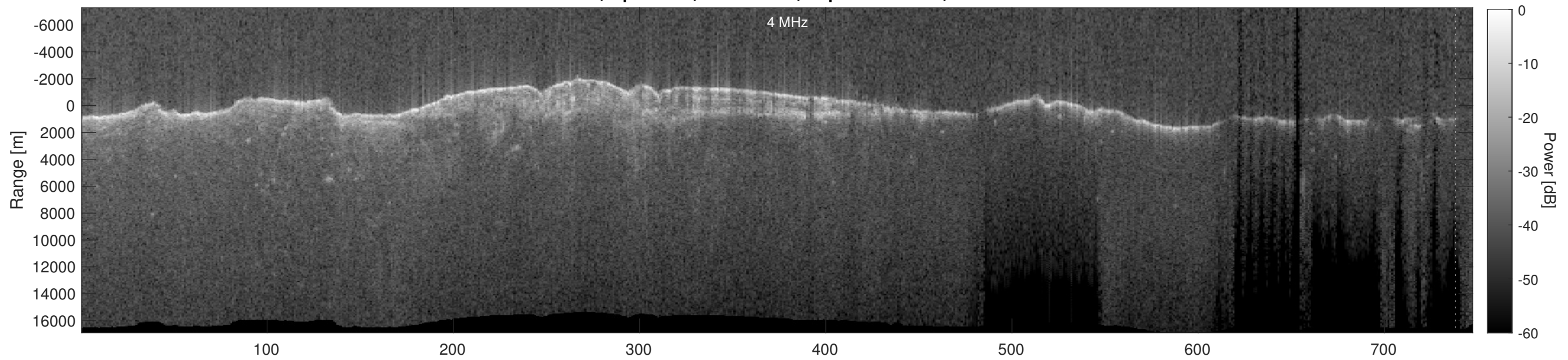
Orbit 6486, Depth-Corrected Cluttergram
