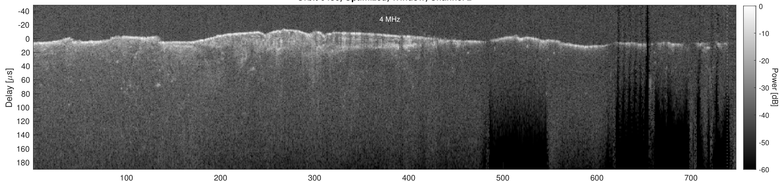
Orbit 6486, Cluttergram
