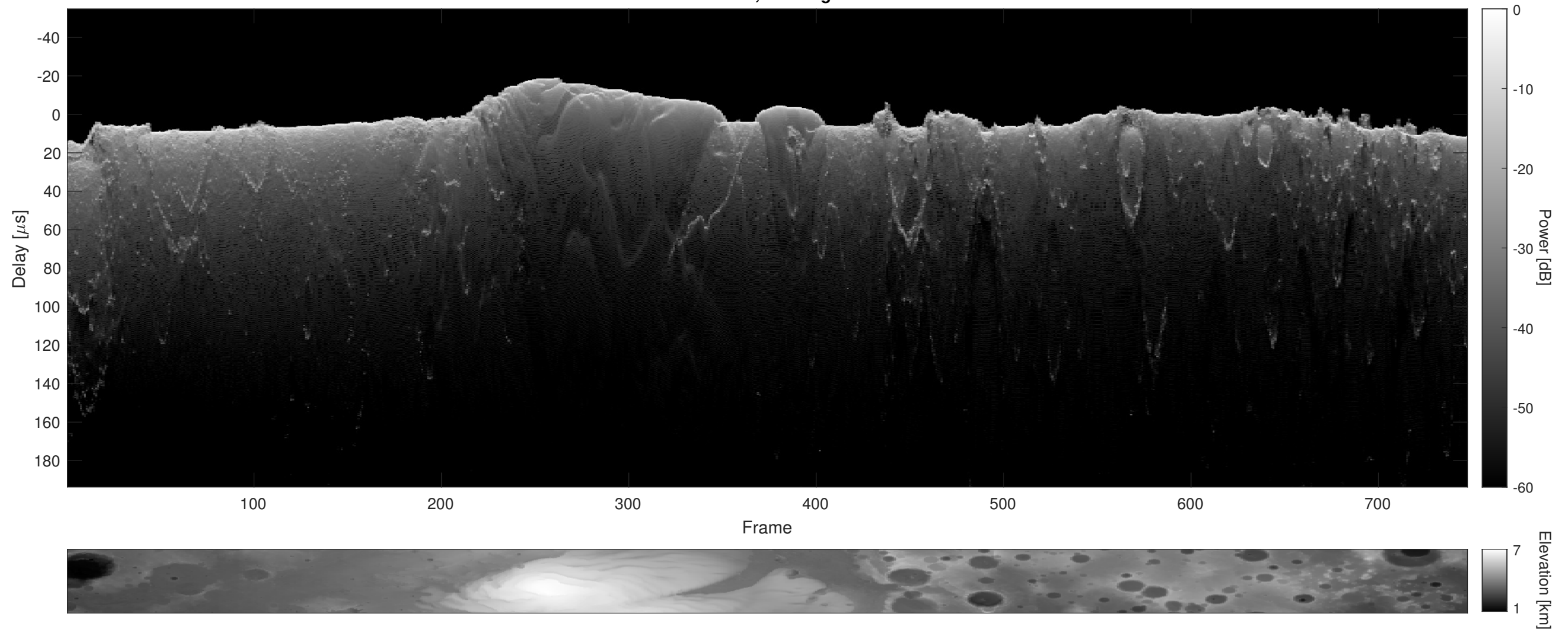
Orbit 6487, Cluttergram
