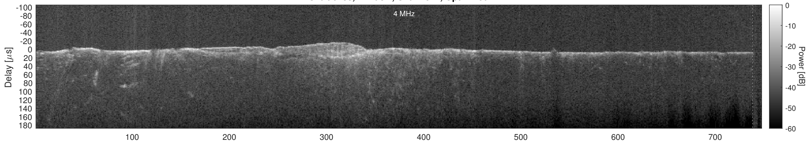
Orbit 6488, Cluttergram
