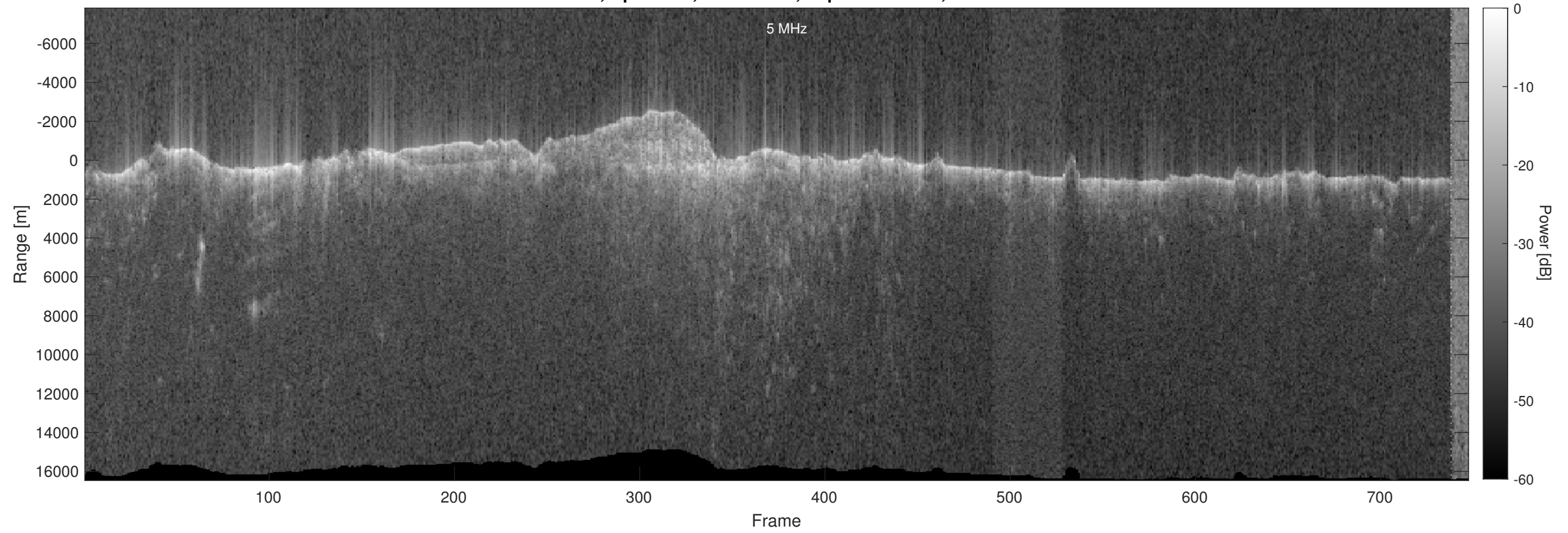
Orbit 6488, Optimized, No Window, Depth-Corrected, Channel 2
