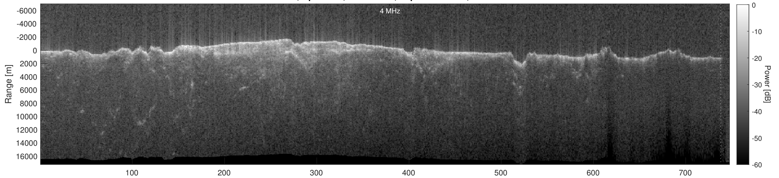
Orbit 6489, Depth-Corrected Cluttergram
