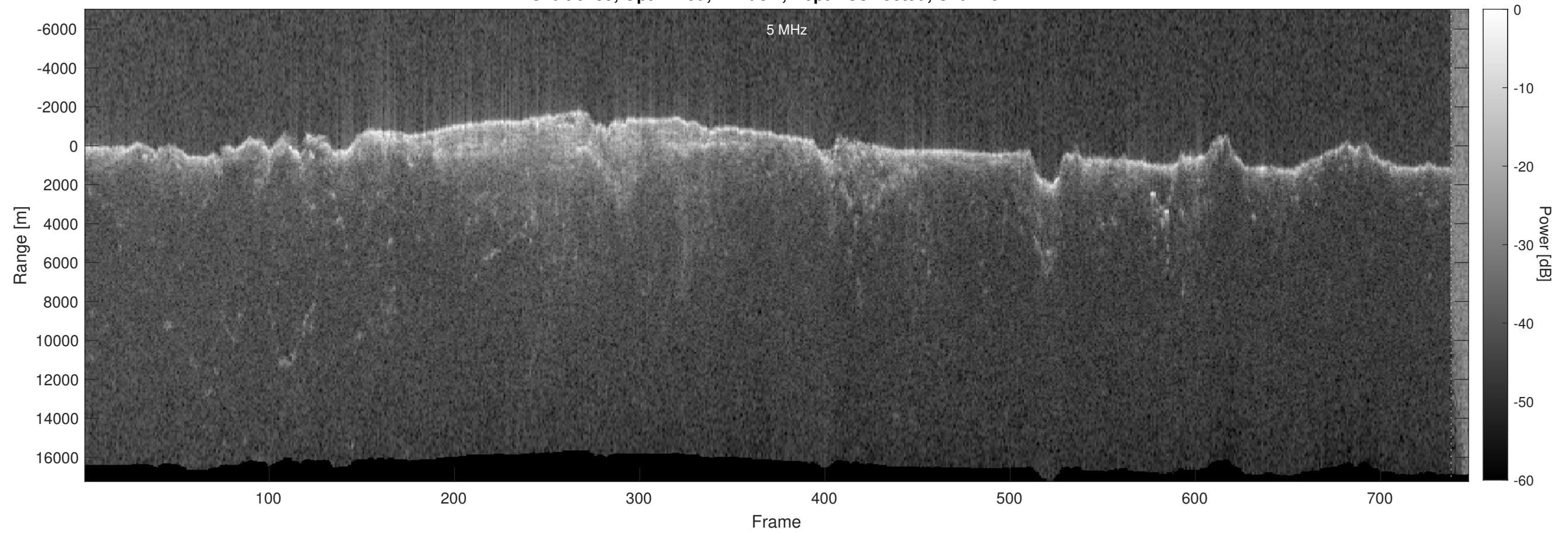
Orbit 6489, Optimized, Window, Depth-Corrected, Channel 2
