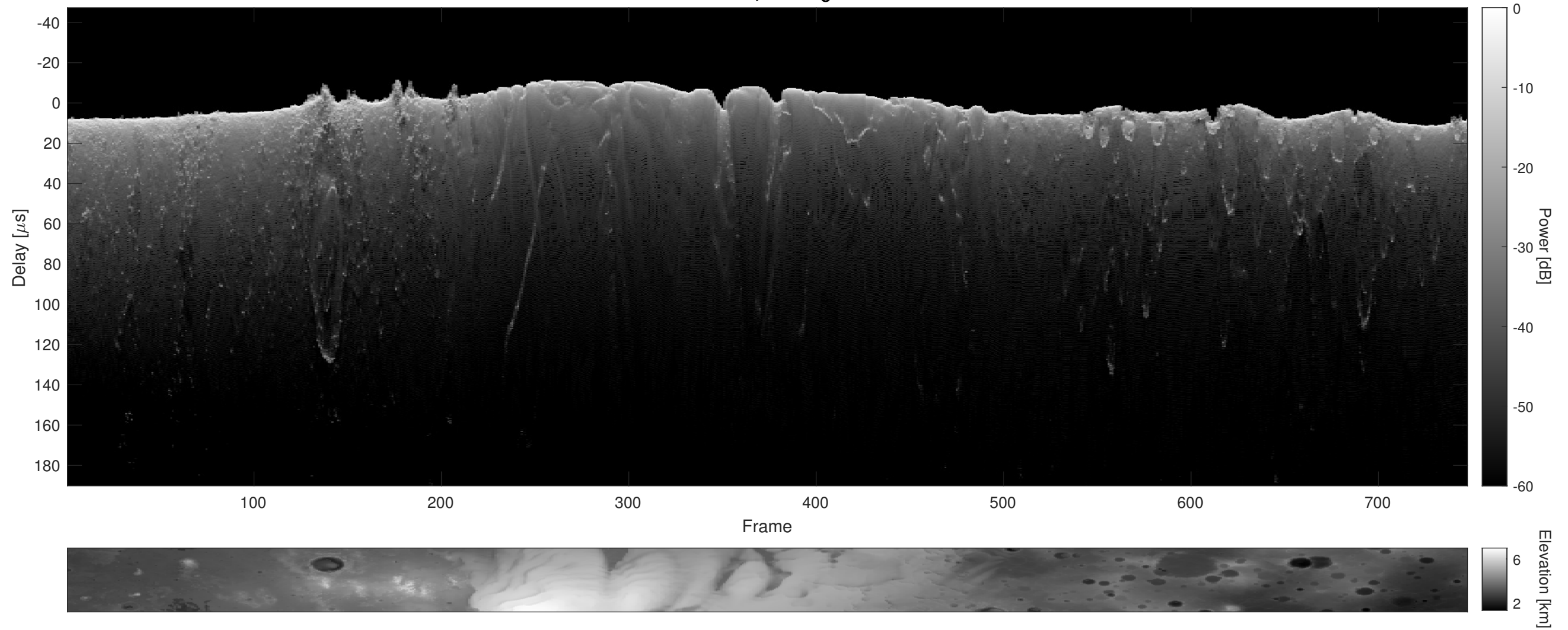
Orbit 6490, Cluttergram
