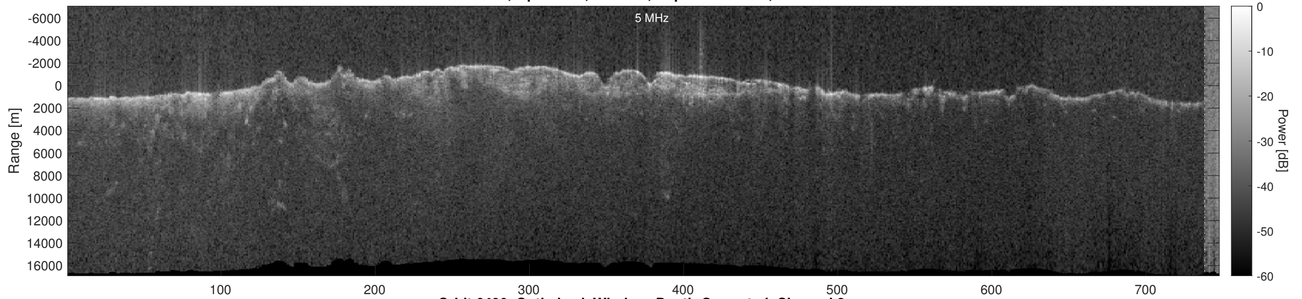
Orbit 6490, Optimized, Window, Depth-Corrected, Channel 2
