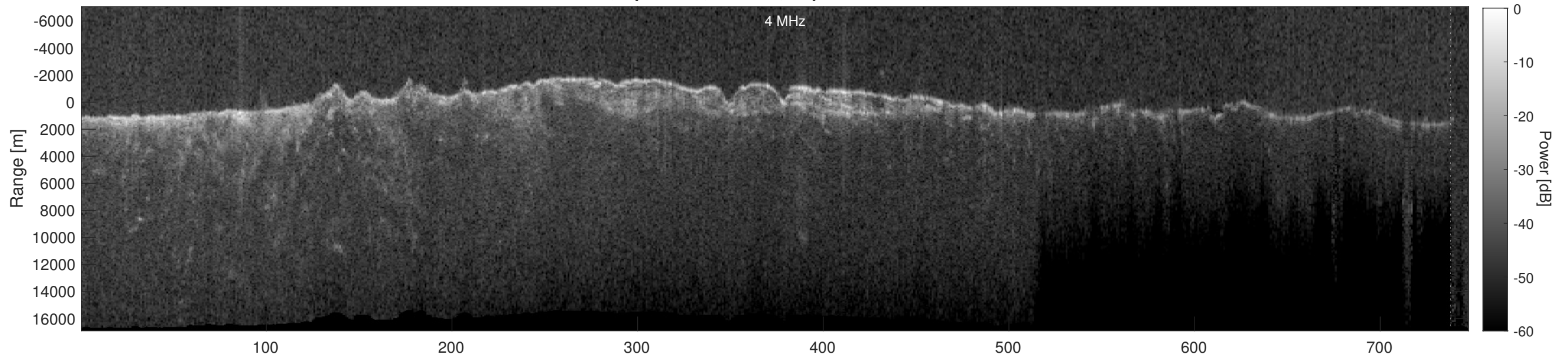
Orbit 6490, Depth-Corrected Cluttergram
