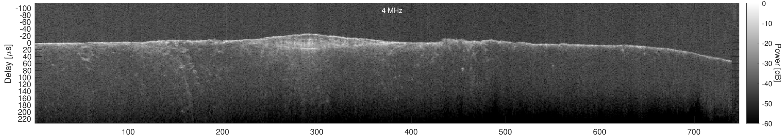
Orbit 6491, Cluttergram
