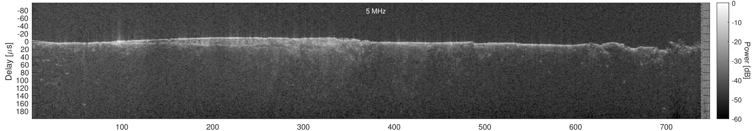
Orbit 6492, Cluttergram
