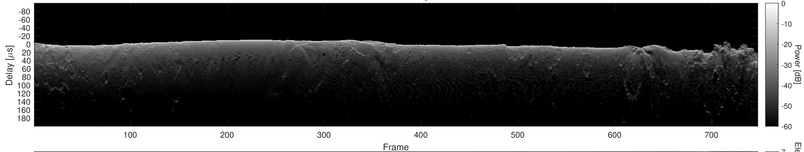
Orbit 6492, Cluttergram
