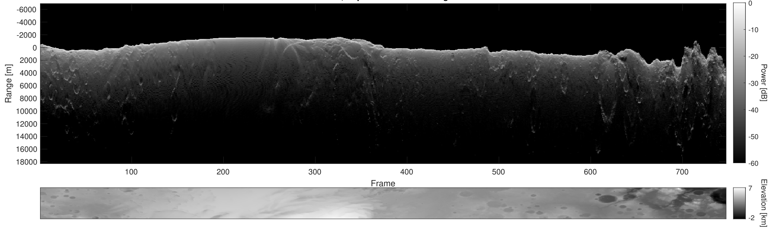
Orbit 6492, Depth-Corrected Cluttergram
