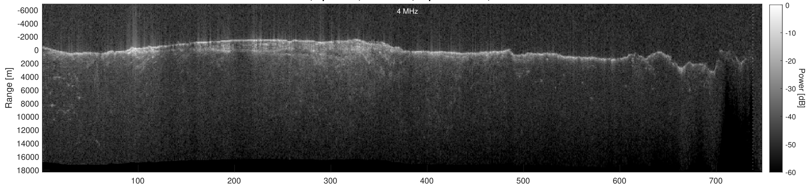
Orbit 6492, Depth-Corrected Cluttergram
