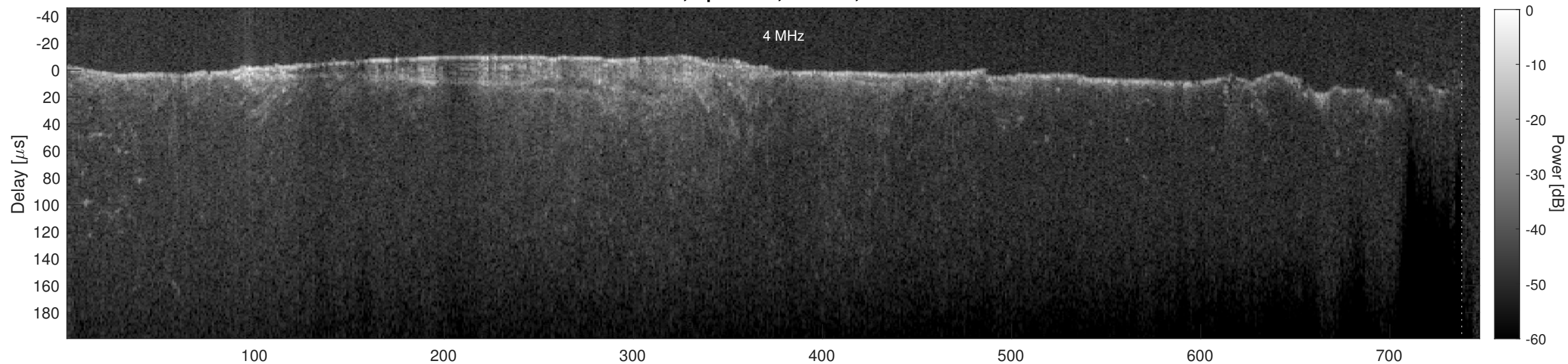
Orbit 6492, Cluttergram
