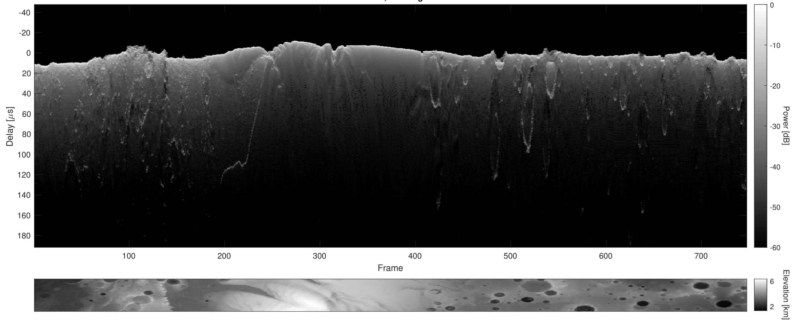
Orbit 6493, Cluttergram
