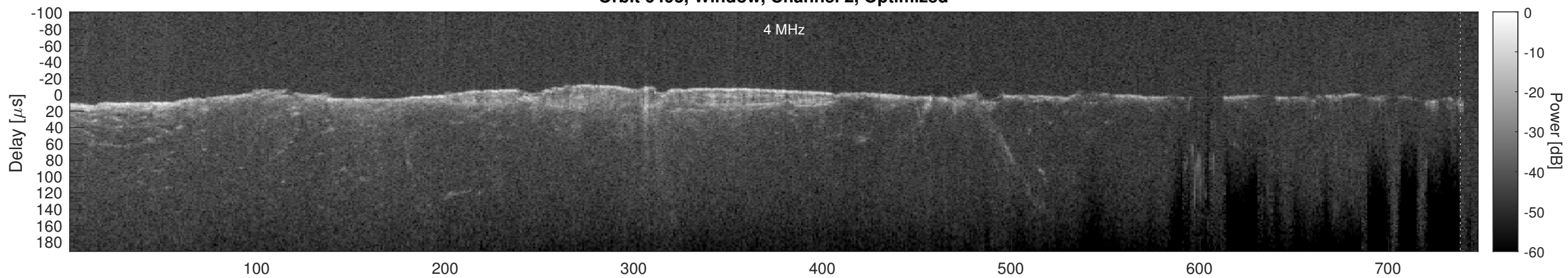
Orbit 6493, Cluttergram
