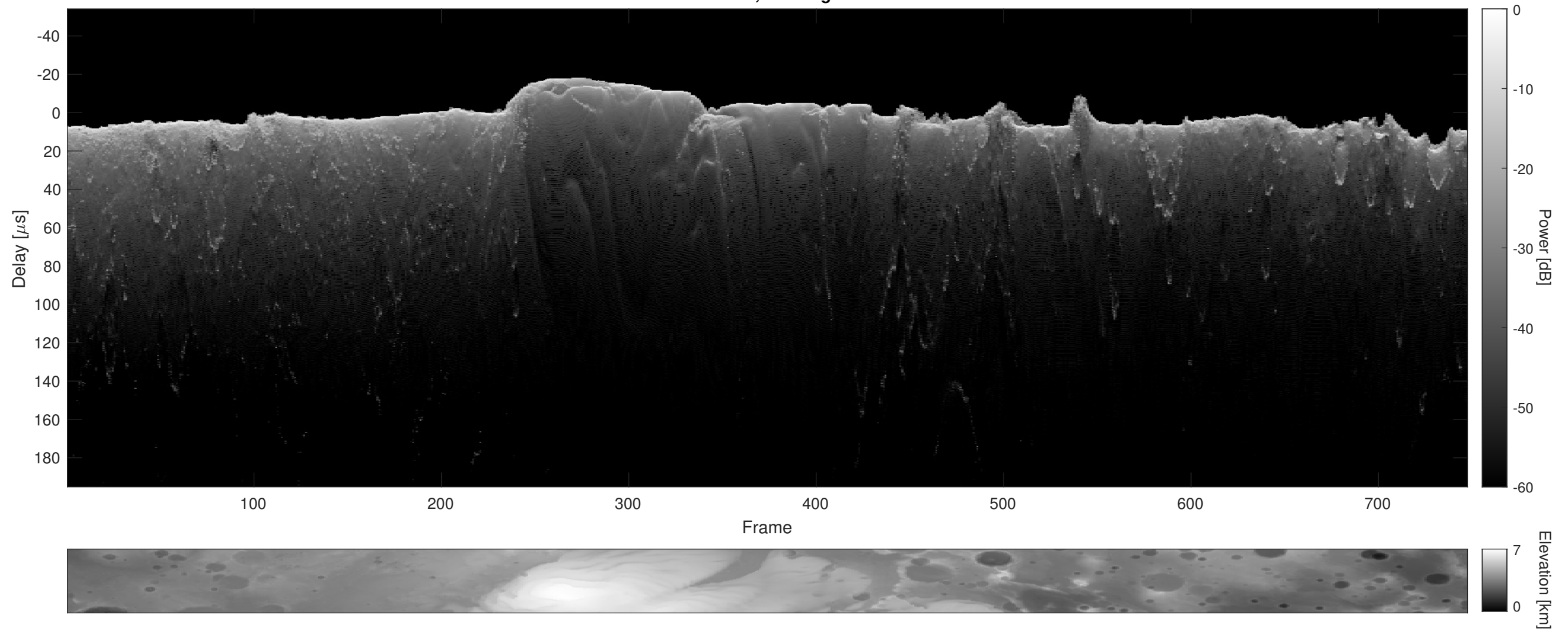
Orbit 6494, Cluttergram
