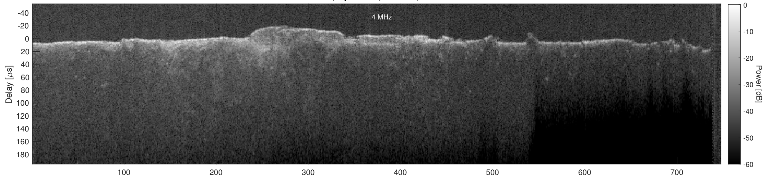
Orbit 6494, Cluttergram
