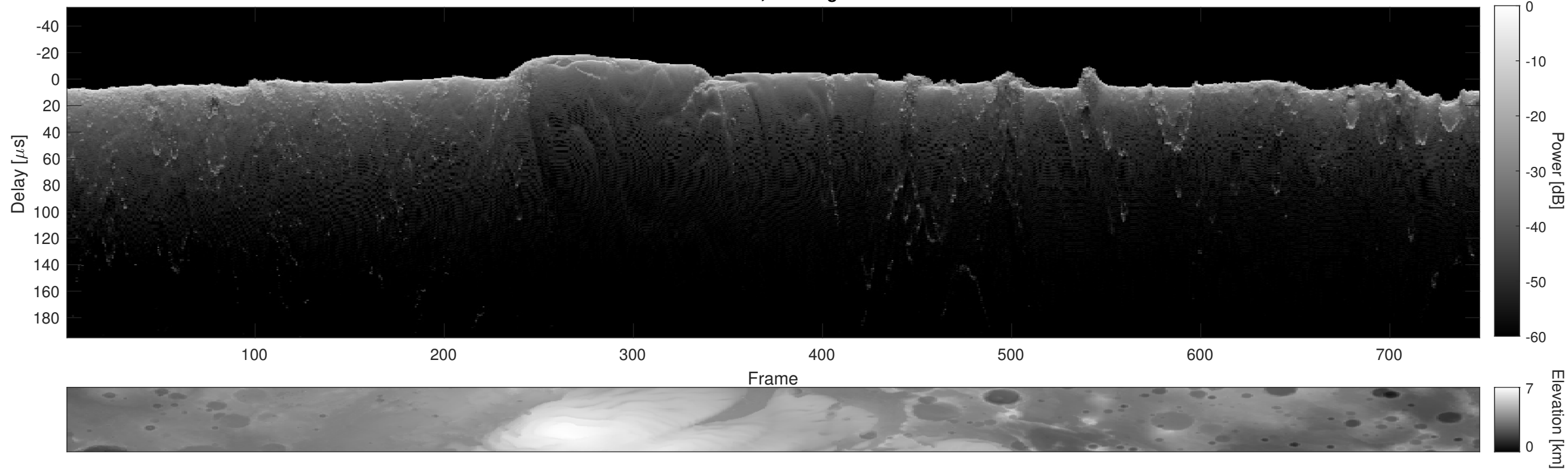
Orbit 6494, Cluttergram
