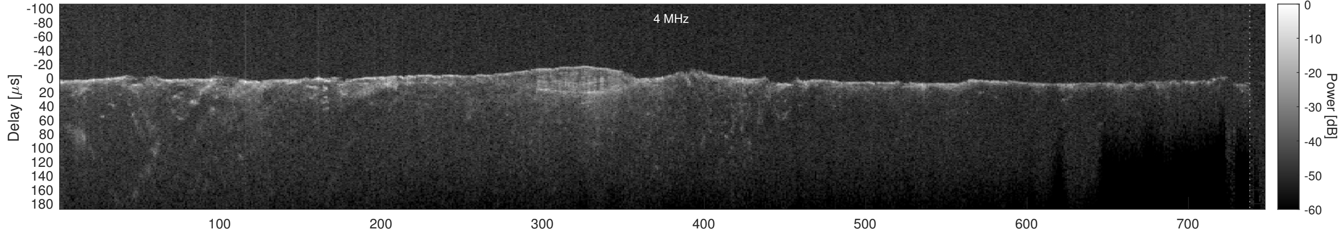
Orbit 6495, Cluttergram
