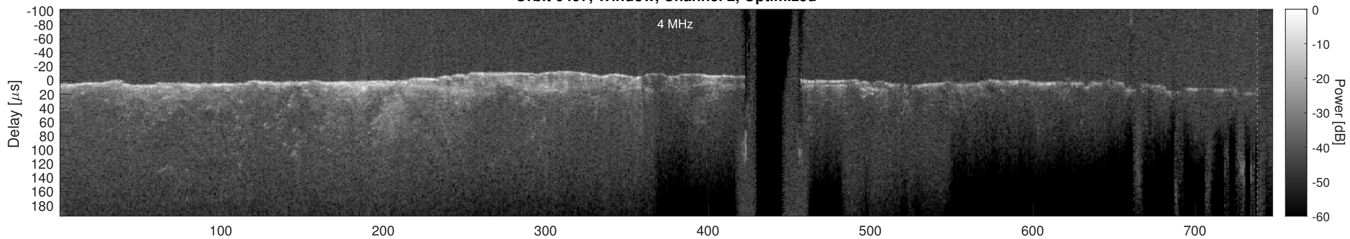
Orbit 6497, Cluttergram
