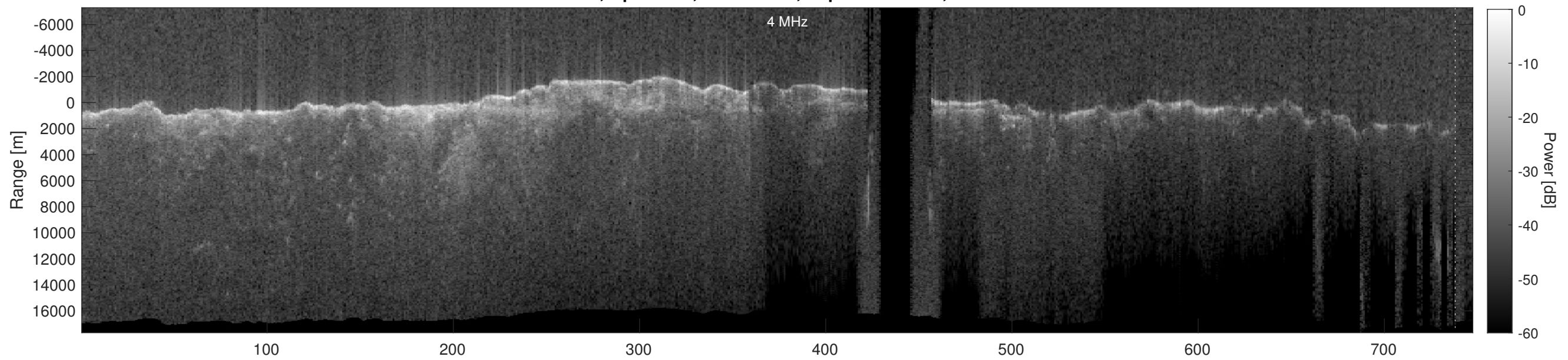
Orbit 6497, Depth-Corrected Cluttergram
