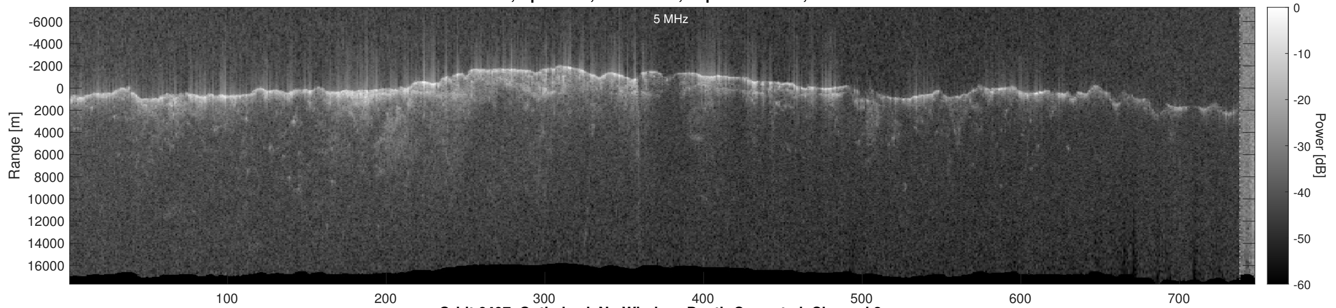
Orbit 6497, Optimized, No Window, Depth-Corrected, Channel 2
