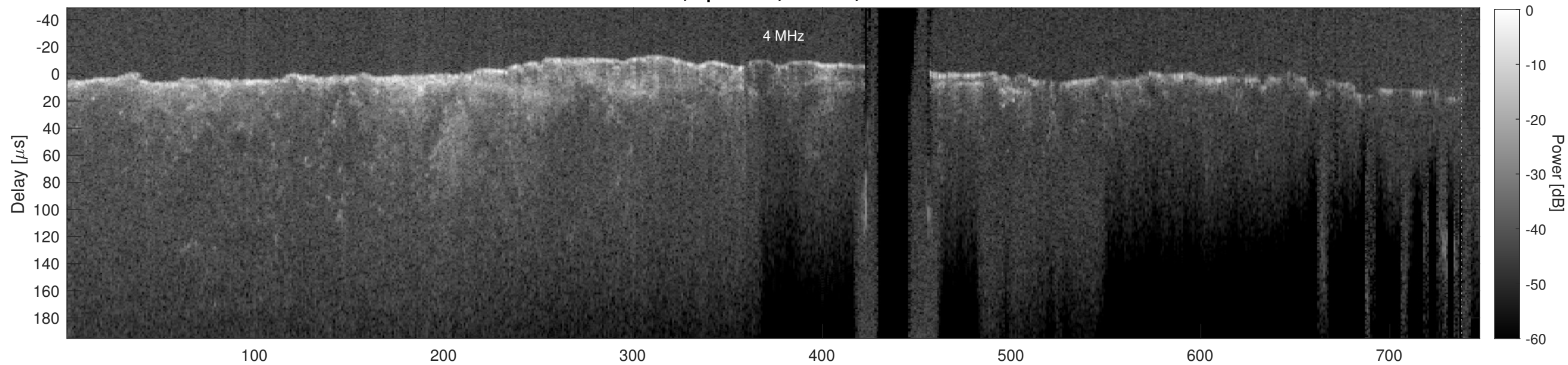
Orbit 6497, Cluttergram
