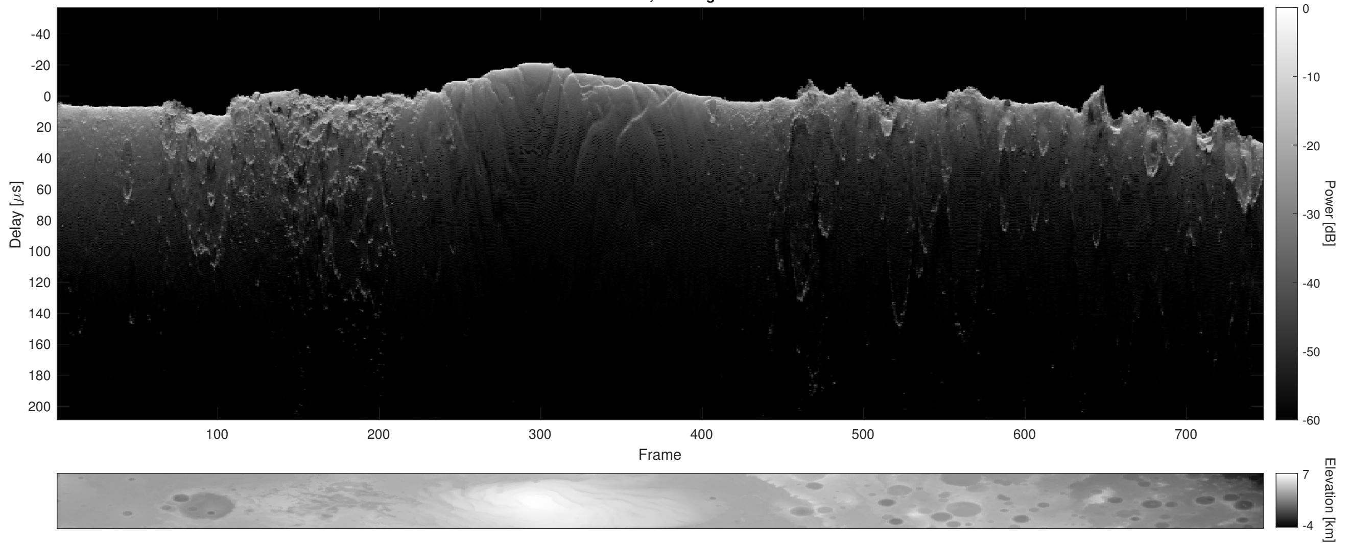
Orbit 6498, Cluttergram
