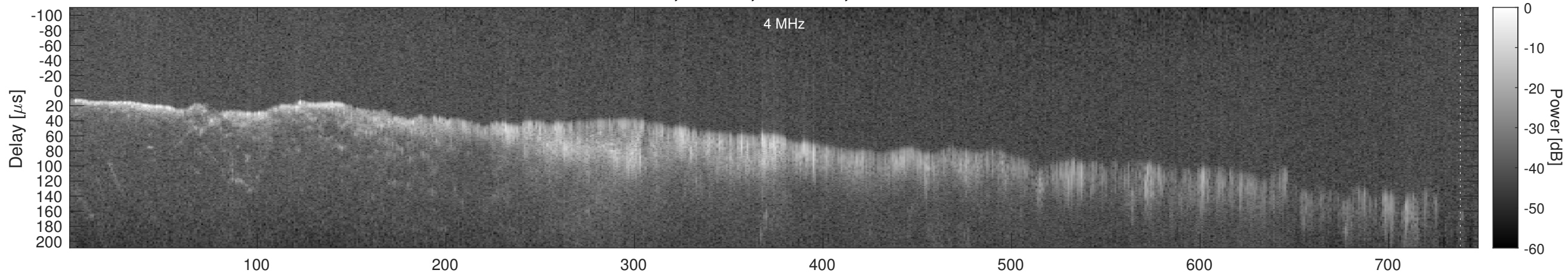
Orbit 6498, Window, Channel 2, Chapman
