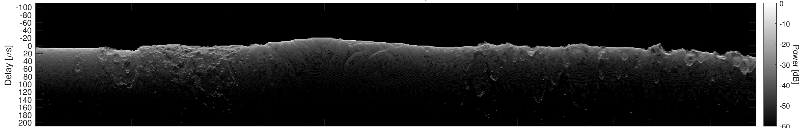
Orbit 6498, Cluttergram
