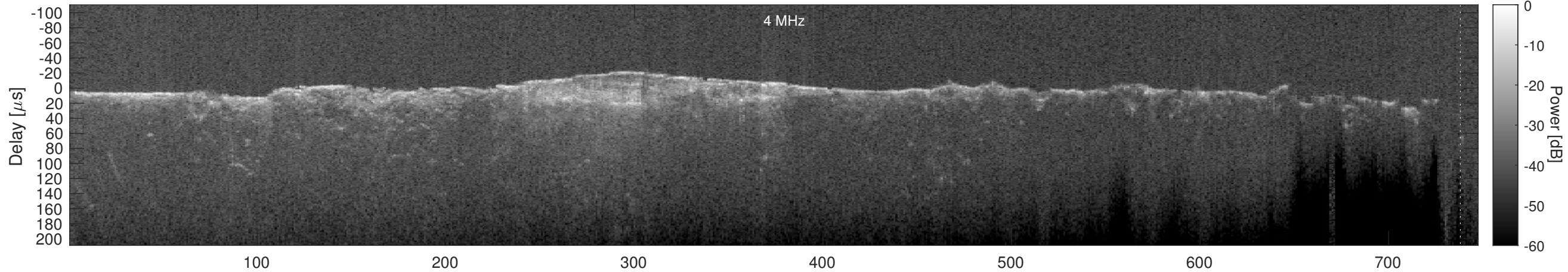
Orbit 6498, Cluttergram
