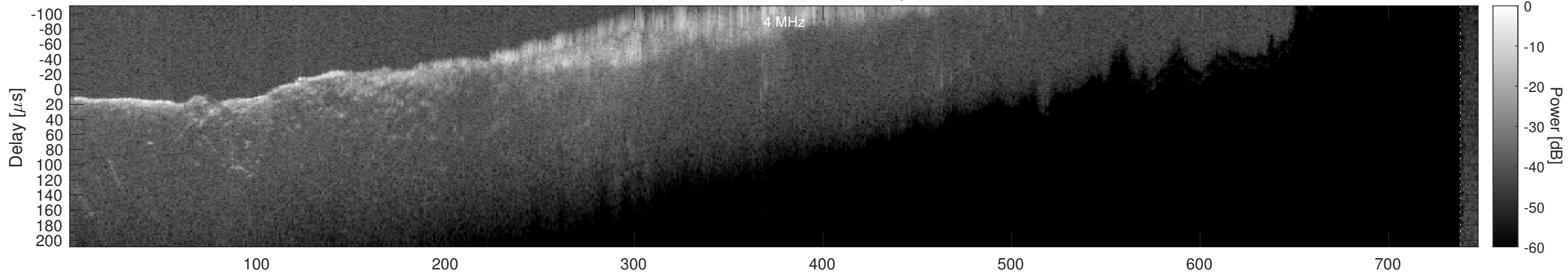
Orbit 6498, Window, Channel 2, Optimized
