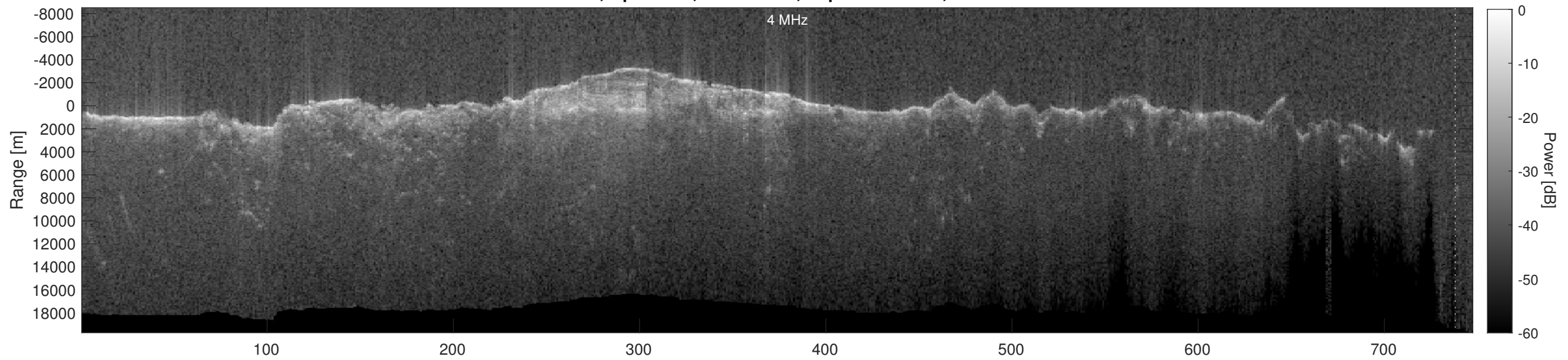
Orbit 6498, Depth-Corrected Cluttergram
