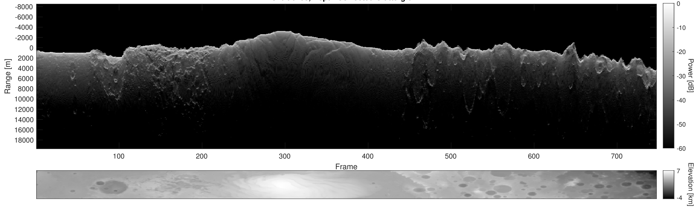
Orbit 6498, Depth-Corrected Cluttergram
