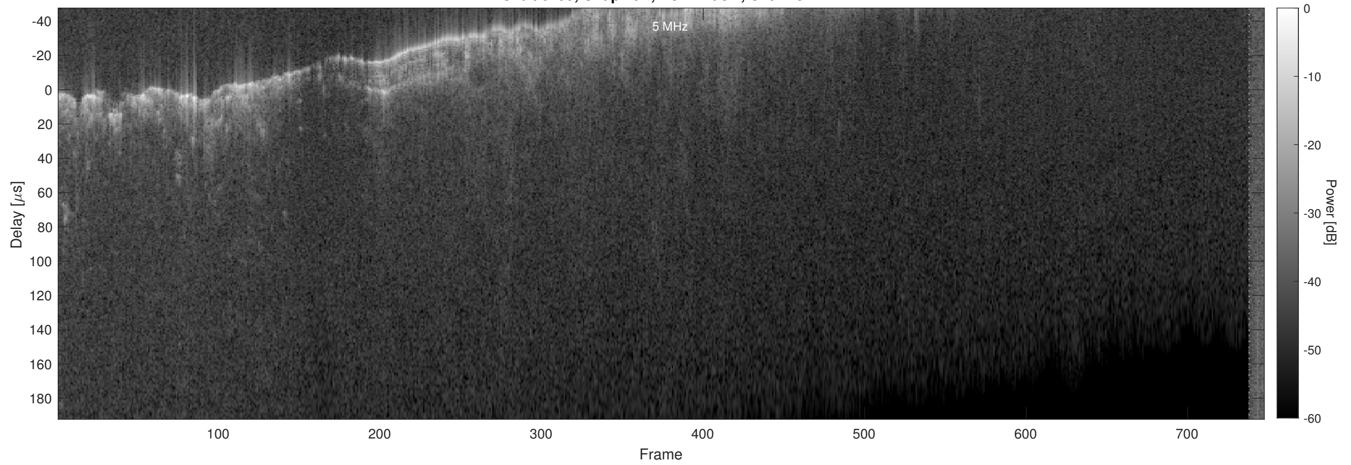
Orbit 6499, Chapman, No Window, Channel 2
