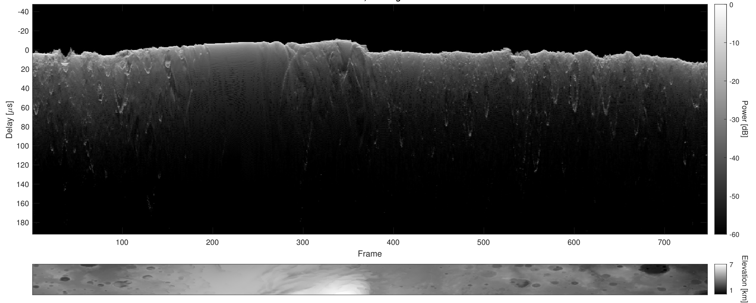
Orbit 6499, Cluttergram
