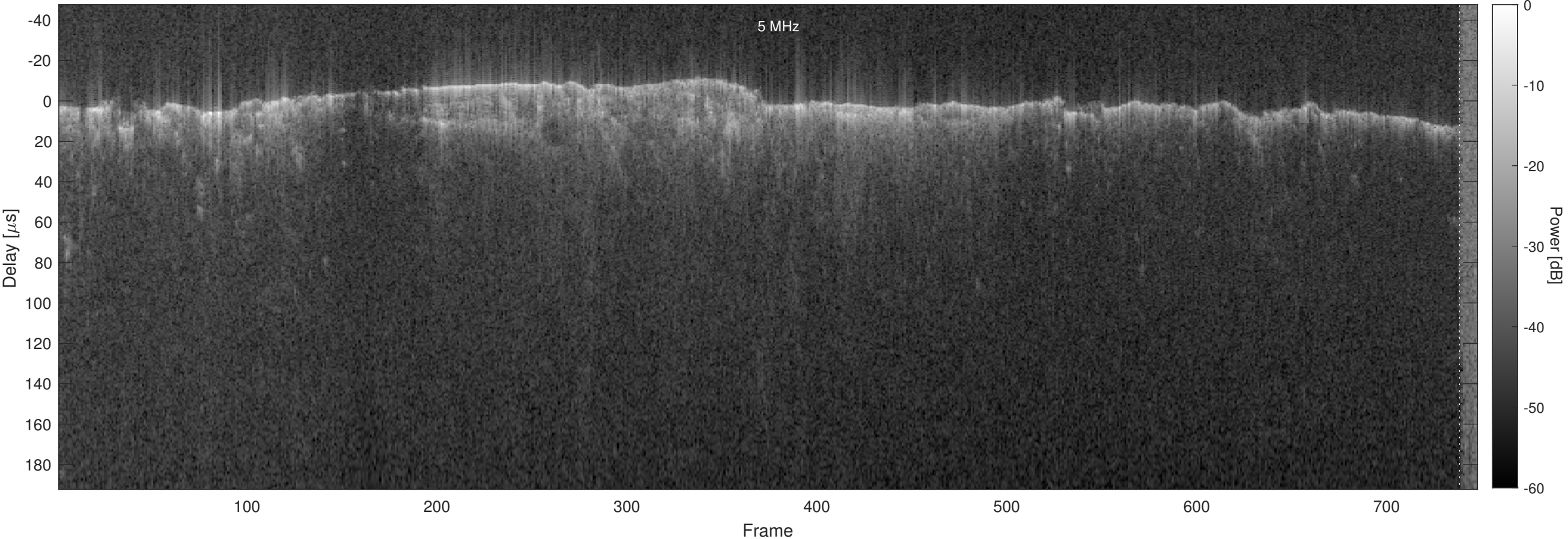
Orbit 6499, Optimized, No Window, Channel 2
