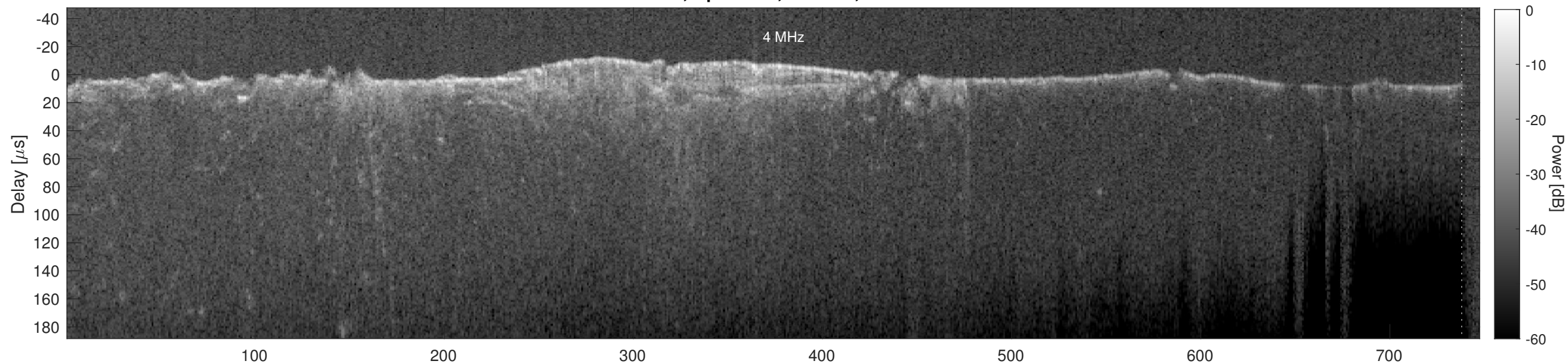
Orbit 6500, Cluttergram
